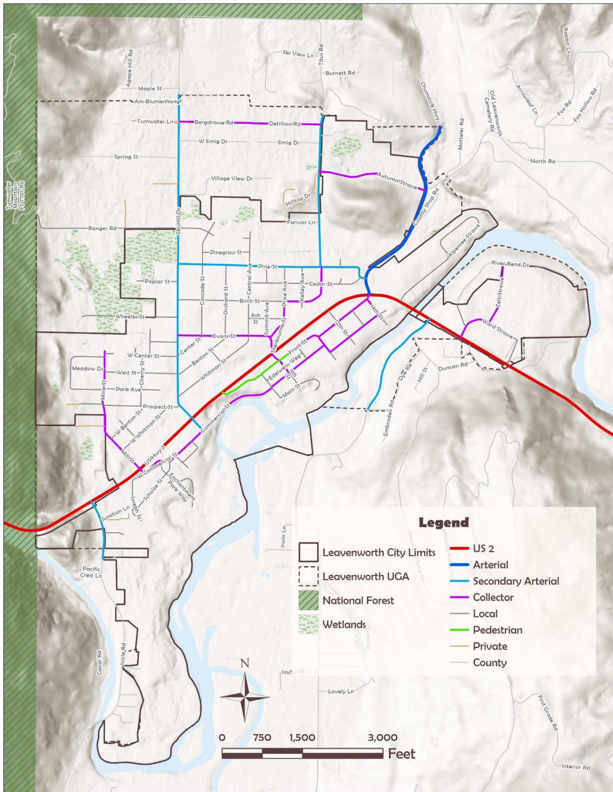
Exhibit 2. Road classification map
